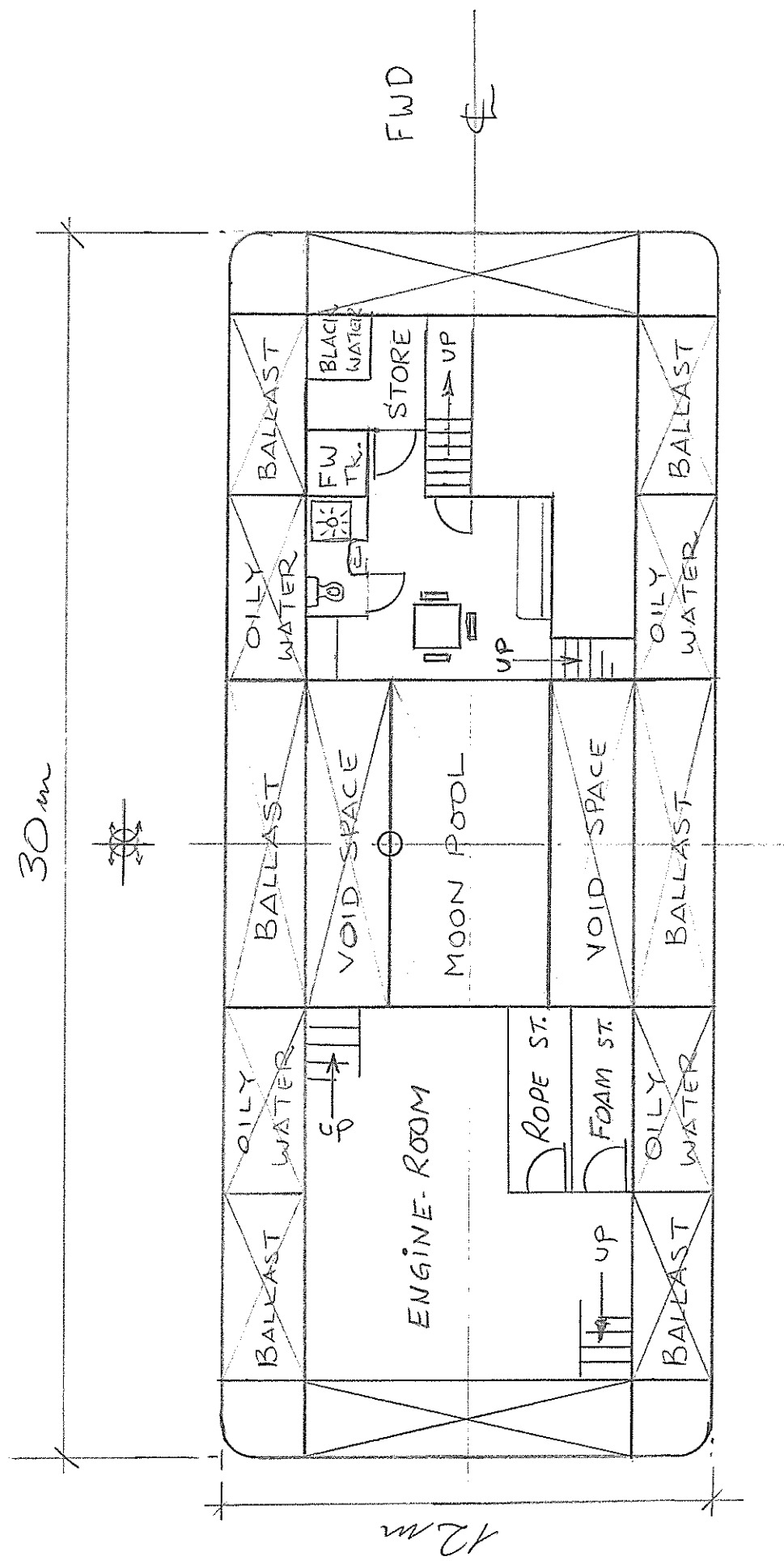
PLAN OF NEW DOLPHIN
